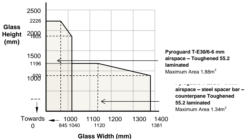
Figure 8 Maximum Permitted Glass
