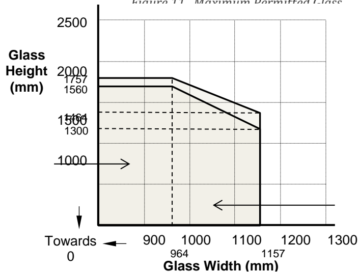
Figure 11 Maximum Permitted Glass
