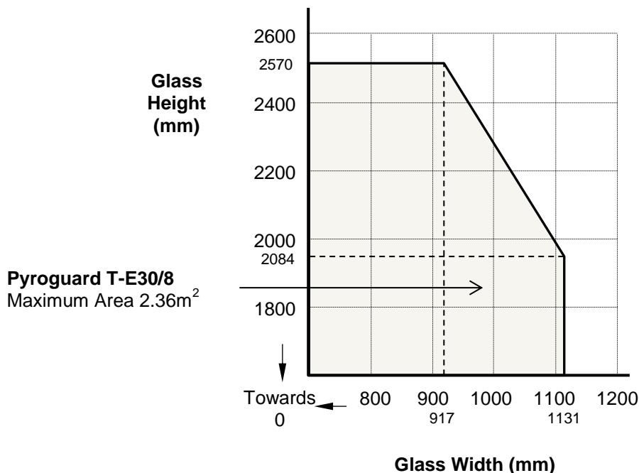
Figure 17. Maximum Permitted Glass Dimensions
