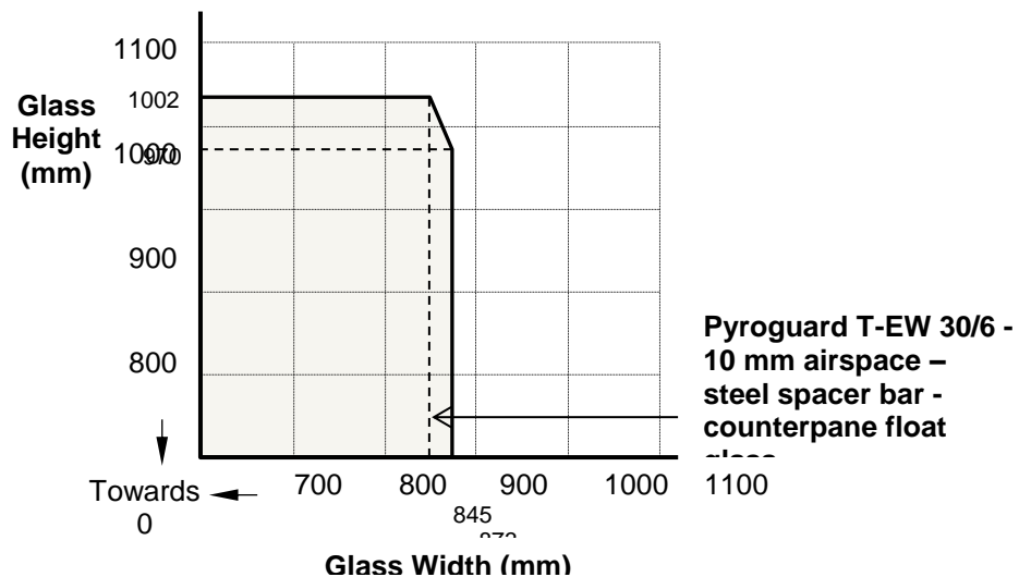
Figure 7. Maximum Permitted Glass
