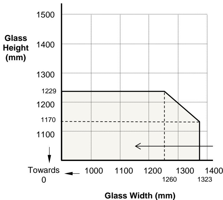
Figure 14 . Maximum Permitted Glass
